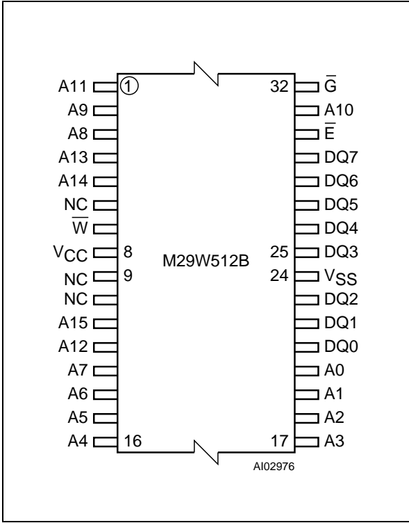
Figure 2A. TSOP Connections
