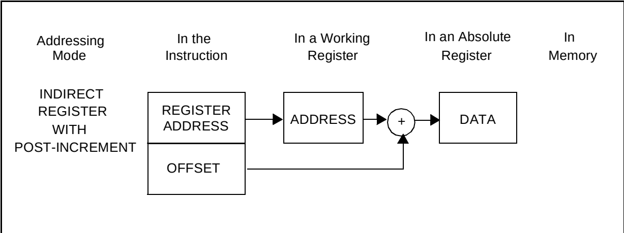
Figure 4. Indexed Register
