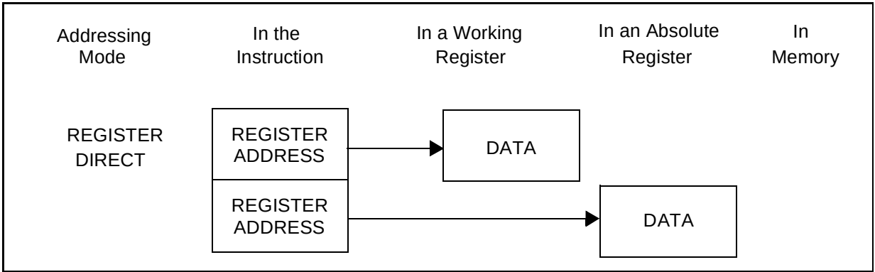
Figure 2. Direct Register
