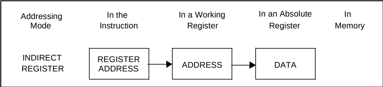
Figure 3. Indirect Register
