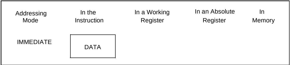
Figure 1. Immediate Register
