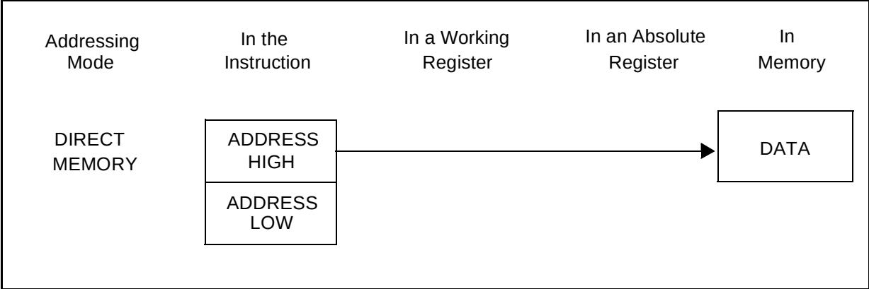
Figure 6. Memory Direct
