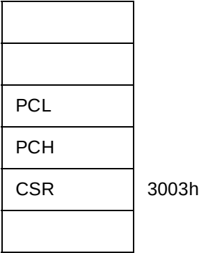
Stack
