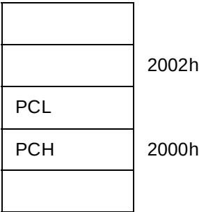
Stack
