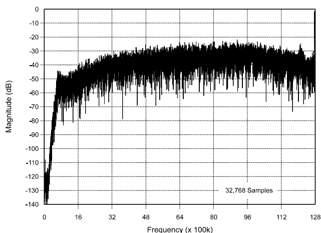
Figure 7. Magnitude versus frequency spectrum of modulator bitstream (MCLK = 25.6 MHz).
