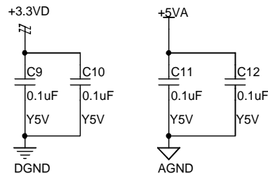
Figure 3. CS4297
