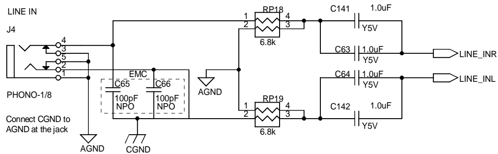
Figure 4. Line Input
