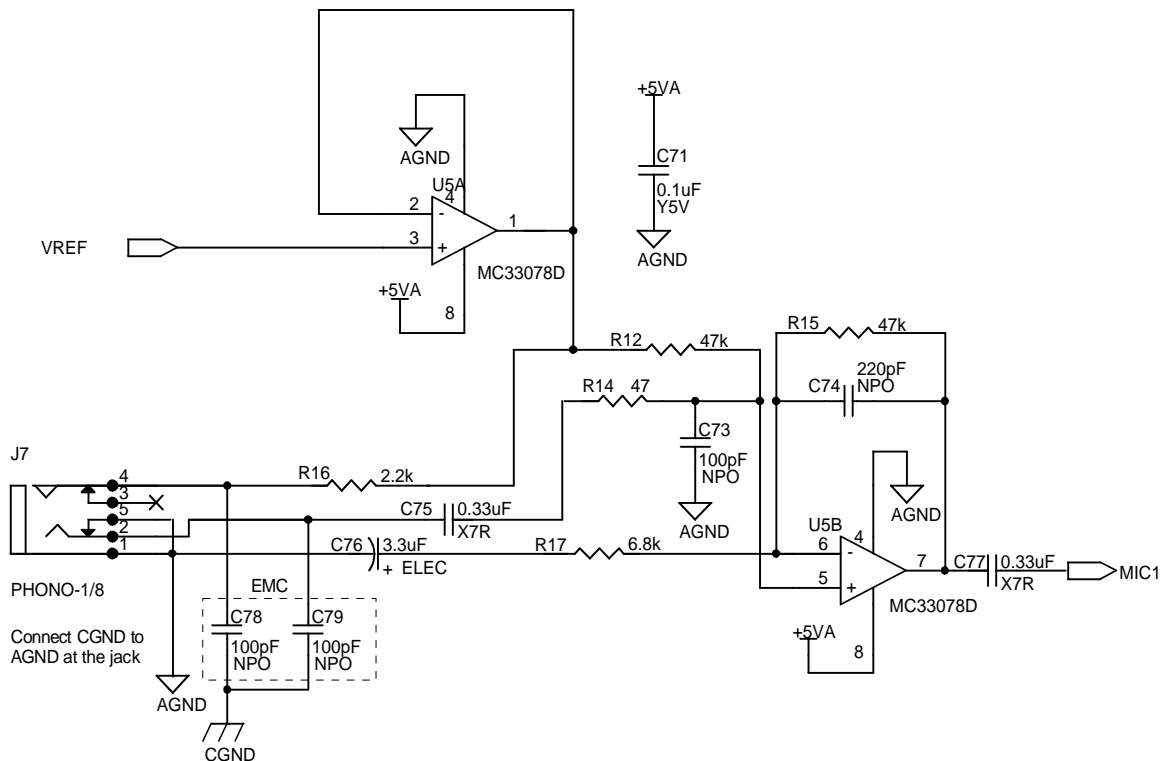
Figure 5. Microphone Input and Amplifier
