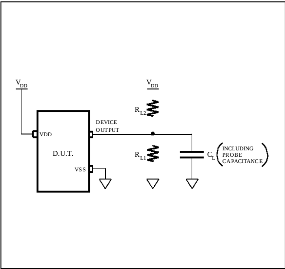
Figure 19. AC Test Circuit (1)
