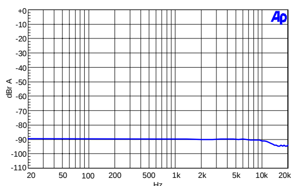
Figure 36. THD+N vs. Frequency (HRM)
