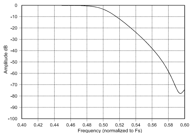
Figure 22. Transition Band
