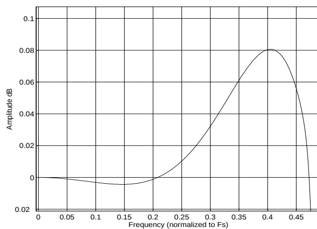
Figure 20. Passband Ripple
