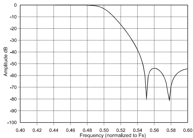
Figure 18. Transition Band
