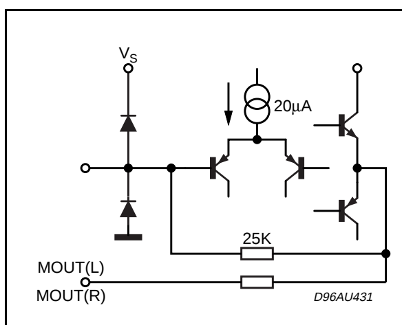
PINS: 20, 25
