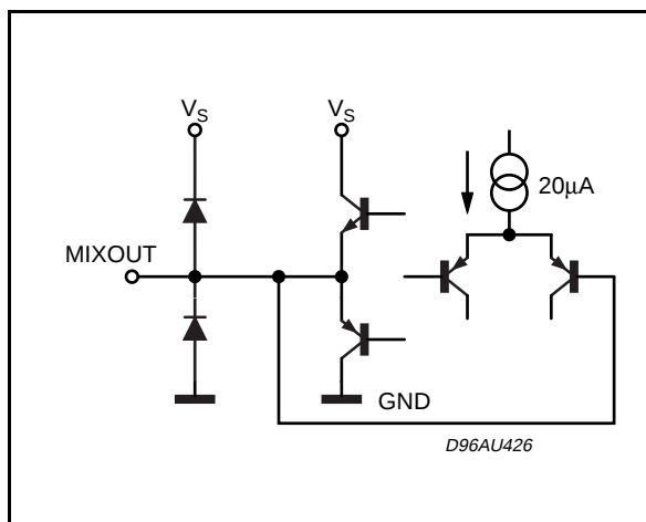
PINS: 15, 17
