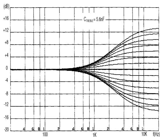
Figure 7: Treble response
