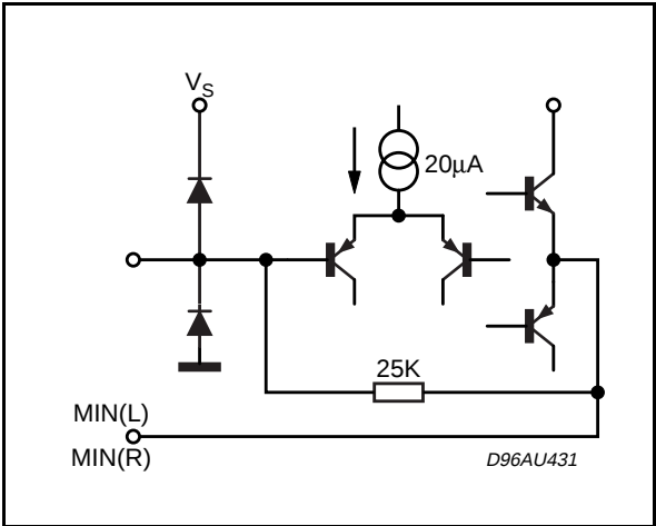
PINS: 19, 26
