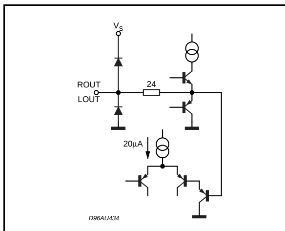
PINS: 5, 6
