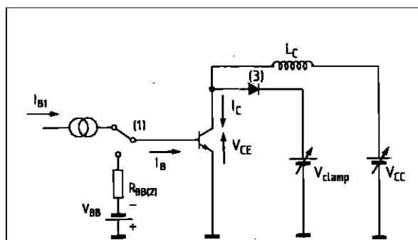
(1) Fast electronic switch (2) Non-inductive load
