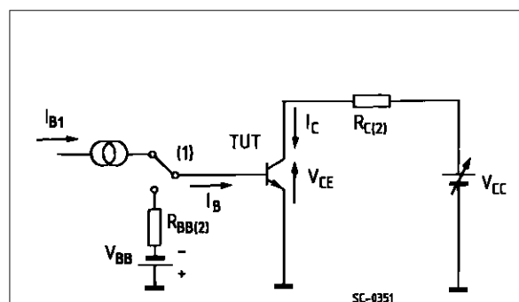
(1) Fast electronic switch
