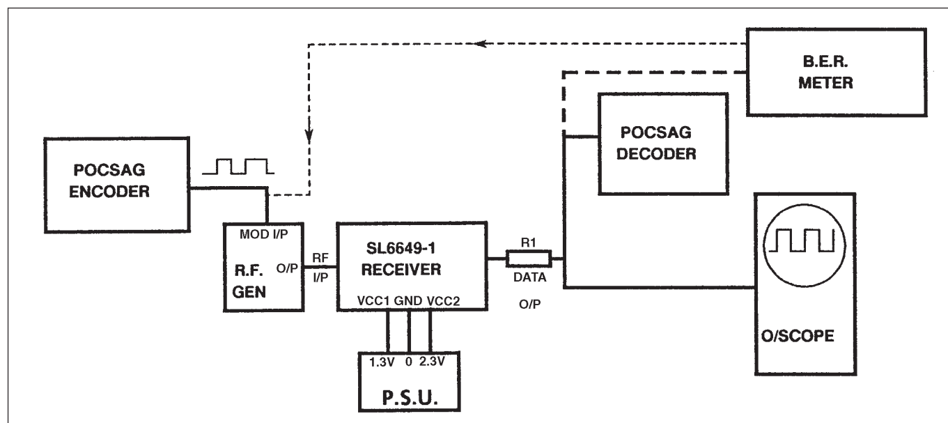
Figure 11: Test System
