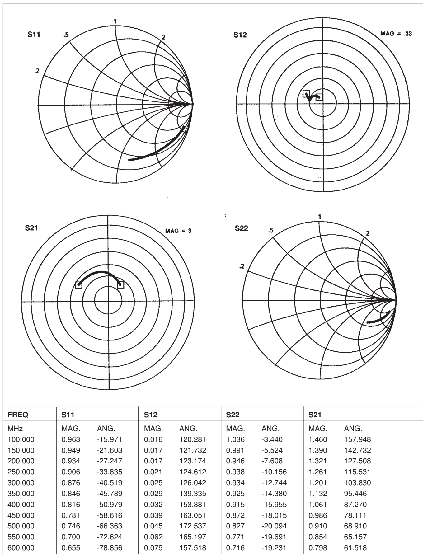
Figure 8: RF Amplifier
