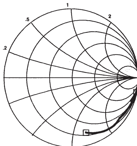
Figure 10: SL6649-1 Mixer LO input pins 26 and 27
