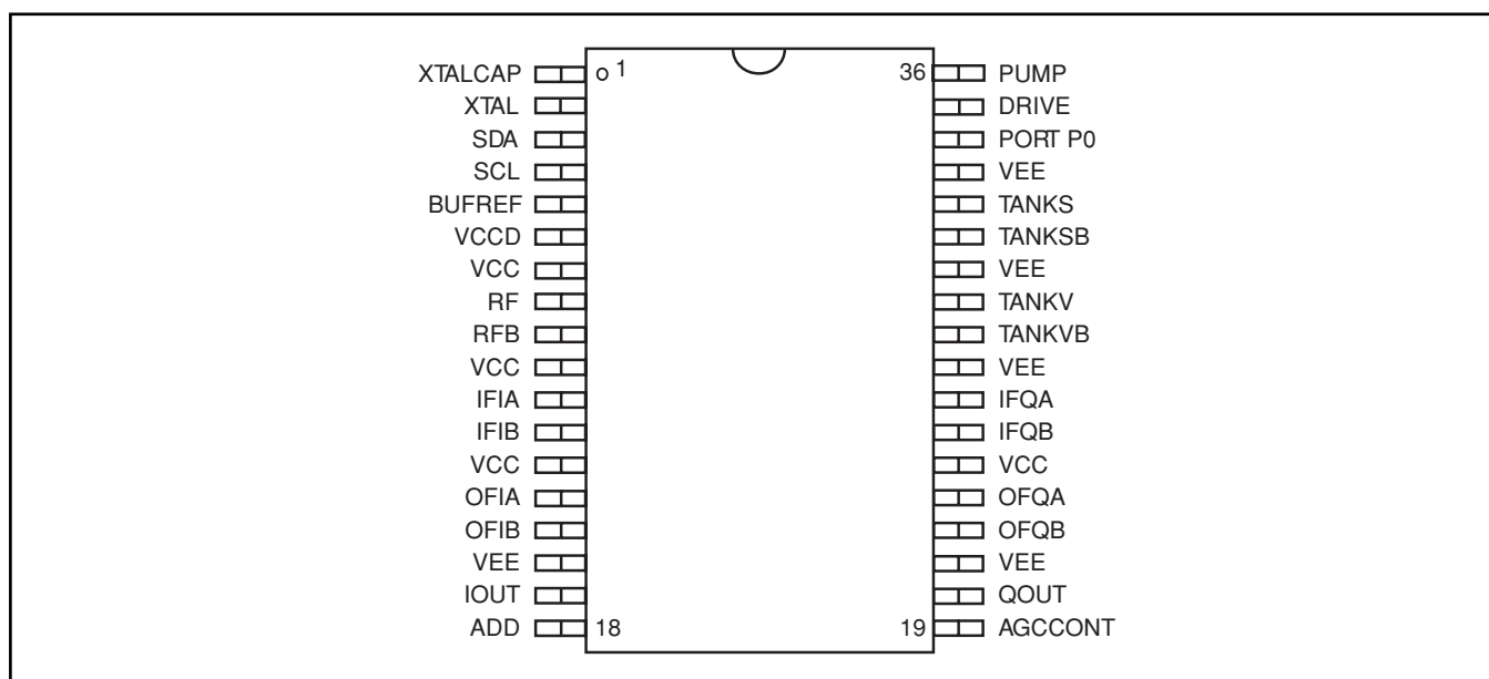
Figure1. Pin connections
