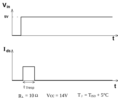
Figure 6 Definition of t_{Tresp}
