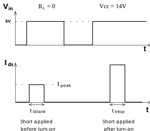
Figure 4 Definition of I_{peak} , t_{blank} , t_{resp}
