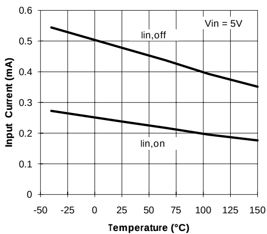
Figure 12 Input Current vs. Temperature
