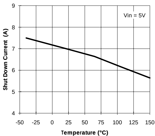
Figure 10 Over-Current Shutdown Threshold vs. Temperature
