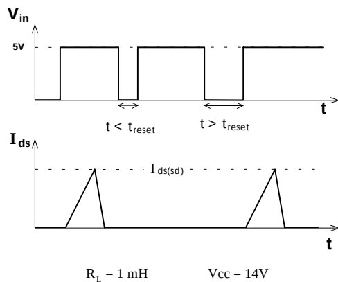
Figure 5 Definition of t_{reset}
