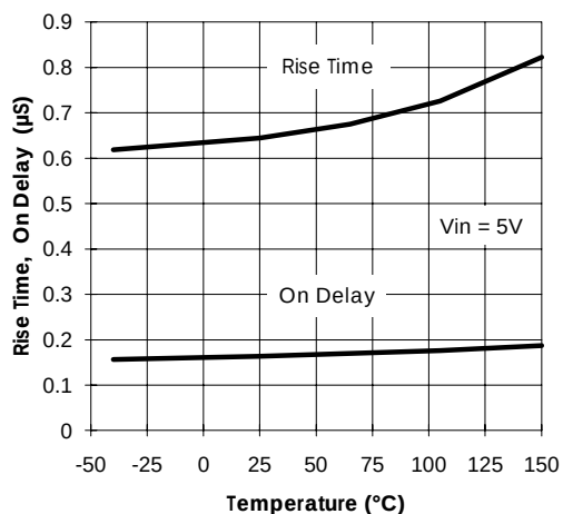
Figure 14 Turn-On Characteristics vs. Temperature
