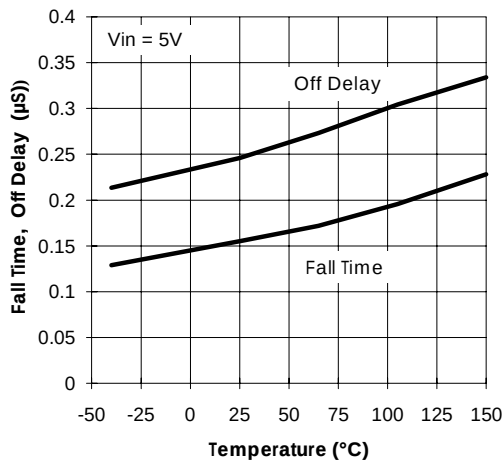
Figure 16 Turn-Off Characteristics vs. Temperature
