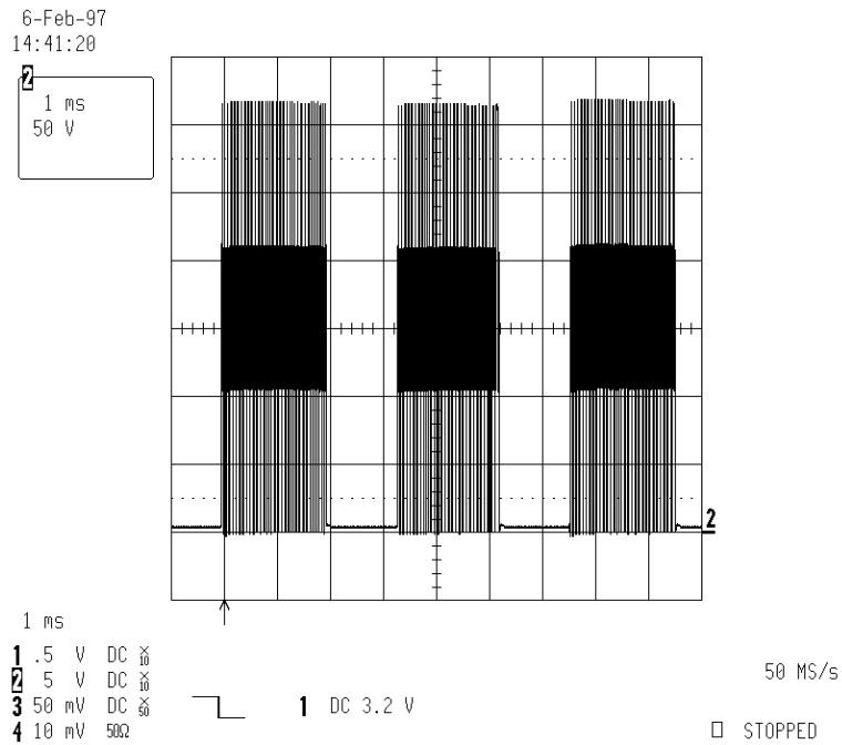
Figure 5 : “Vout” with Lamp Removed ( Burst mode )
