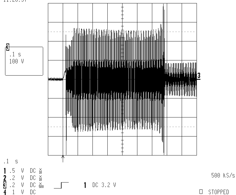
Figure 3 : Lamp Voltage ( Start - Preheat - Running )
