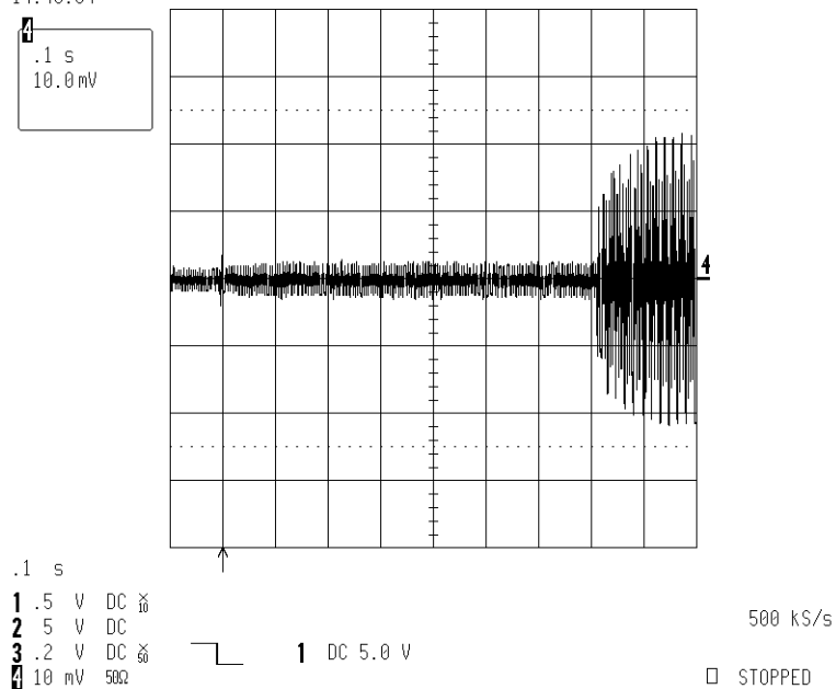
Figure 4 : Lamp Current ( Start - Preheat - Running ) ( 200 mA/div )
