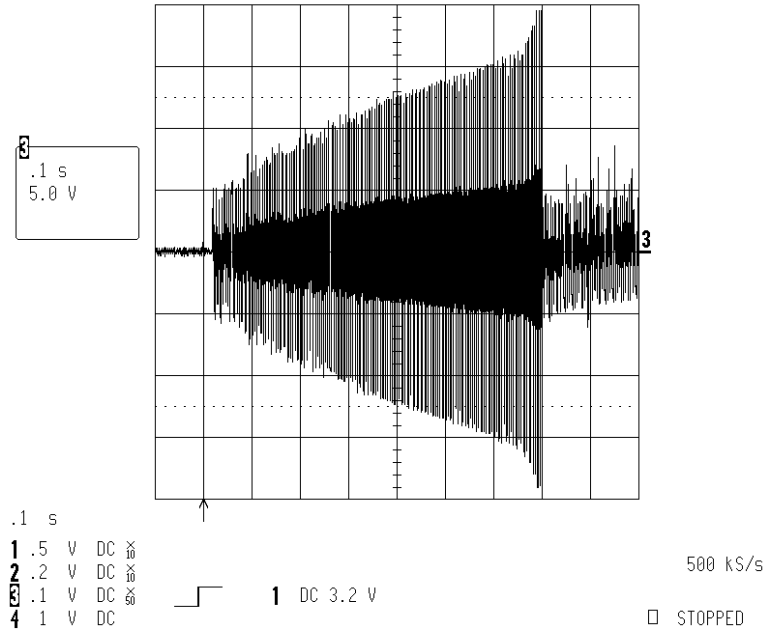
Figure 1 : Cathode Voltage (Start - Preheat - Running)
