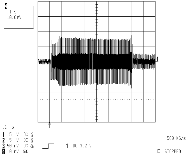
Figure 2 : Cathode Current (Start - Preheat - Running) ( 500 mA/div )
