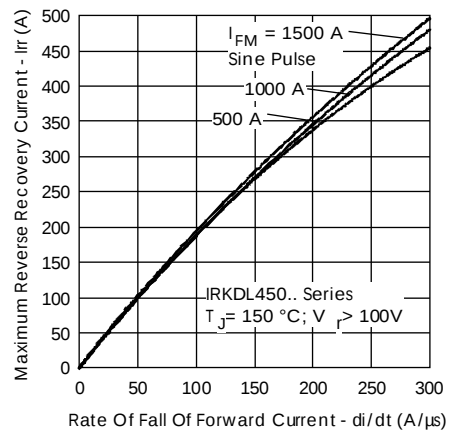
Fig. 11 - Recovery Current Characteristics
