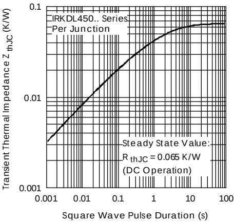
Fig. 13 - Thermal Impedance Z_{thJC} Characteristic
