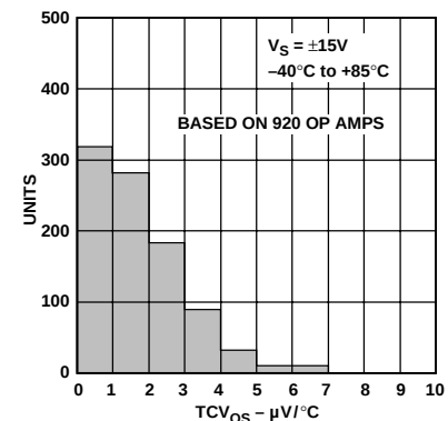
TCV_{OS} Distribution
