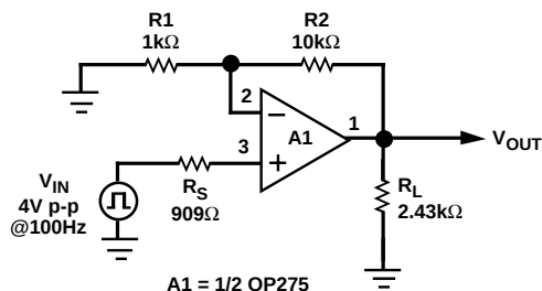
Figure 10. Overload Recovery Time Test Circuit
