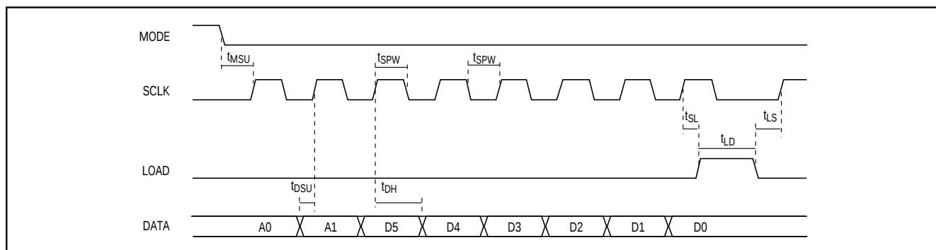
Figure 7. MODE = 0 Timing
