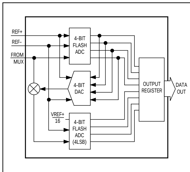
Figure 5. ADC Functional Diagram
