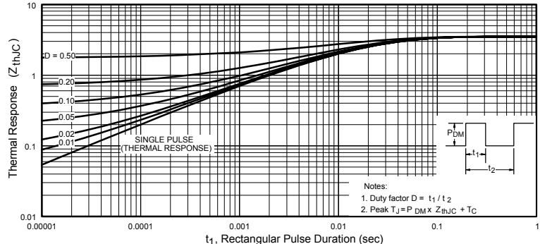
Fig. 4 - Maximum Thermal Impedance Z_{thjC} Characteristics, (per Leg)
