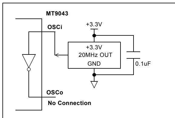
Figure 8 - Clock Oscillator Circuit
