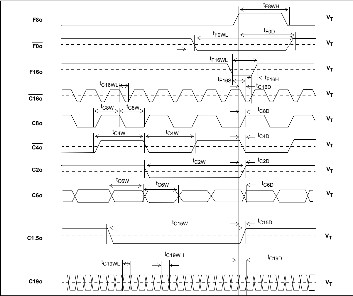
Figure 14 - Output Timing 1
