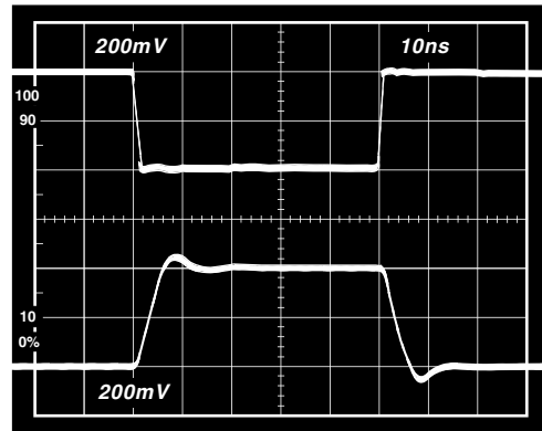
Figure 27. Inverter Small Signal Pulse Response \pm 5 V_S , C_F = 0 \text{ pF} , R_L = 150 \Omega
