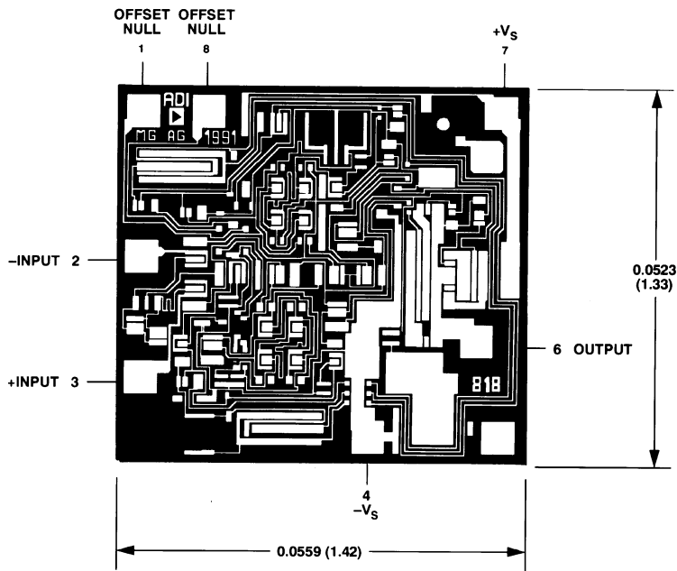
METALIZATION PHOTOGRAPH Dimensions shown in inches and (mm).
