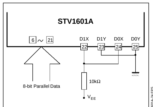
Figure 14 : 8-bit Parallel Input Data (ECL level)
