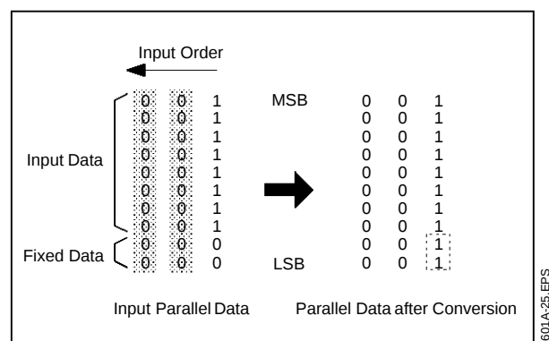
Figure 10 : Conversion from 8-bit TRS to 10-bit TRS
