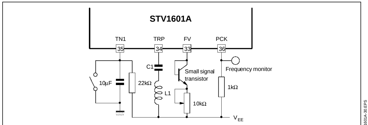
Figure 20 : VCO Temperature Compensation and Free Running Adjustment
