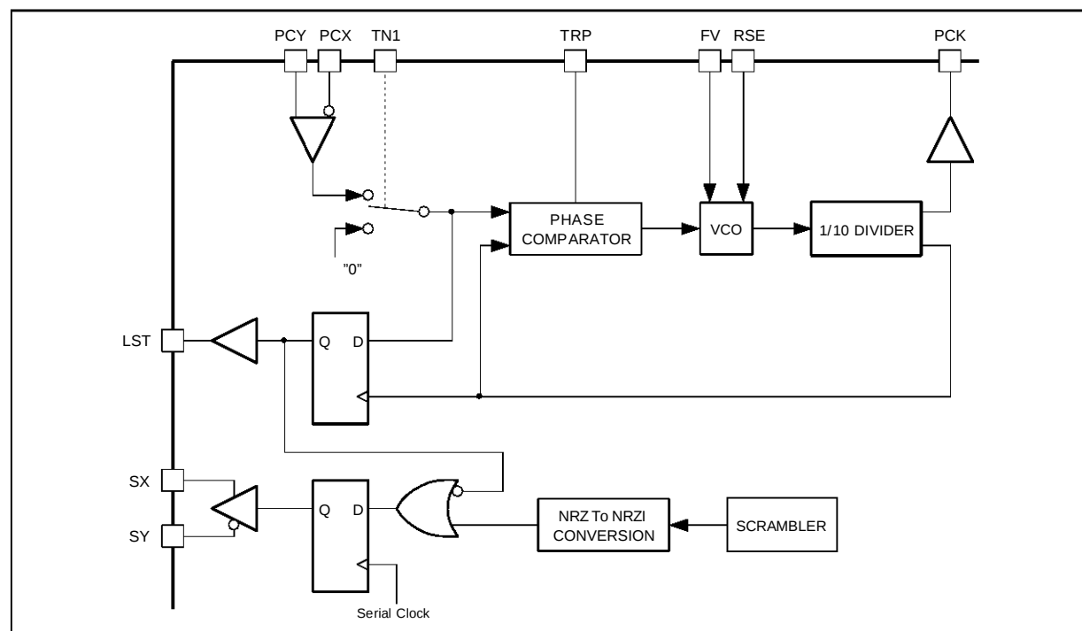
Figure 13 : PLL and Serial Output Control Block
