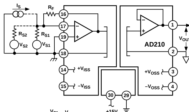
Figure 4. Summing or Current Input Configuration
