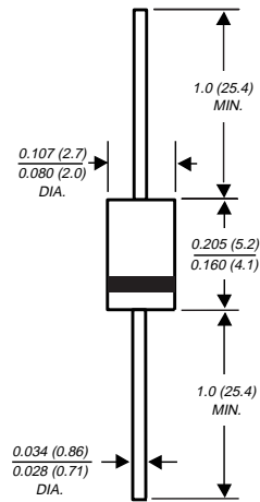
DO-204AL
