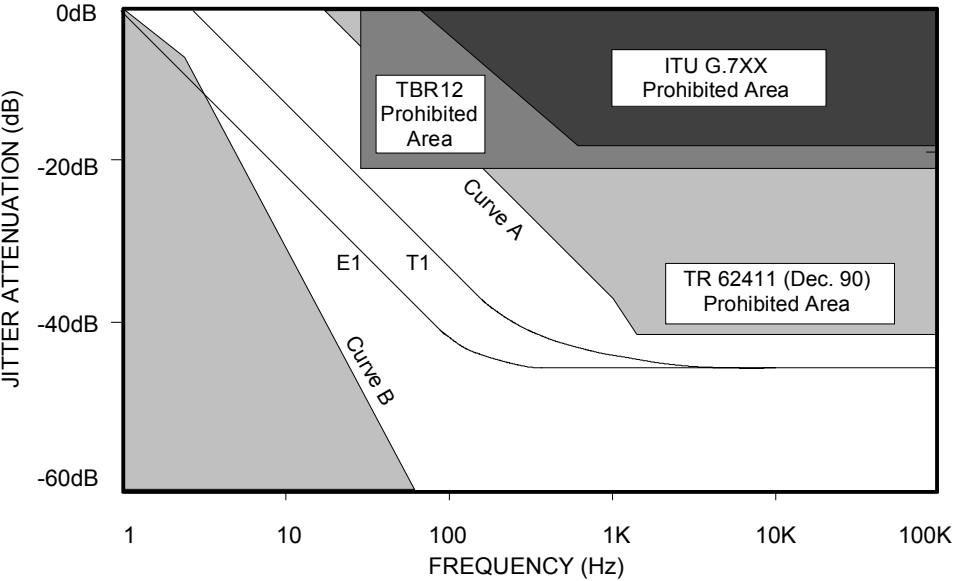
JITTER ATTENUATION Figure 9-7
