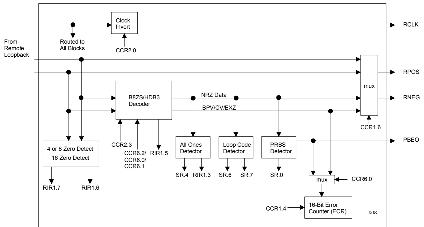
RECEIVE LOGIC Figure 3-2
