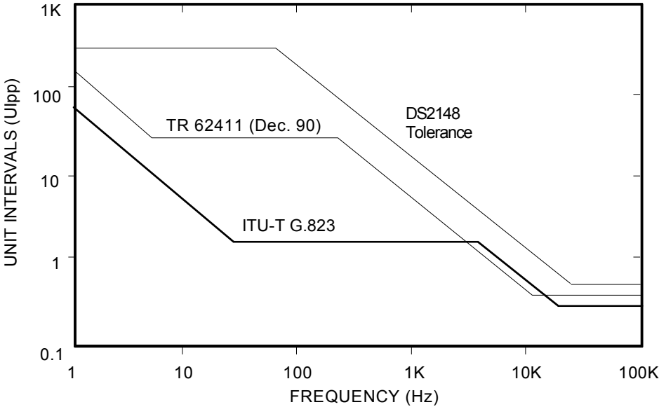
JITTER TOLERANCE Figure 9-6
