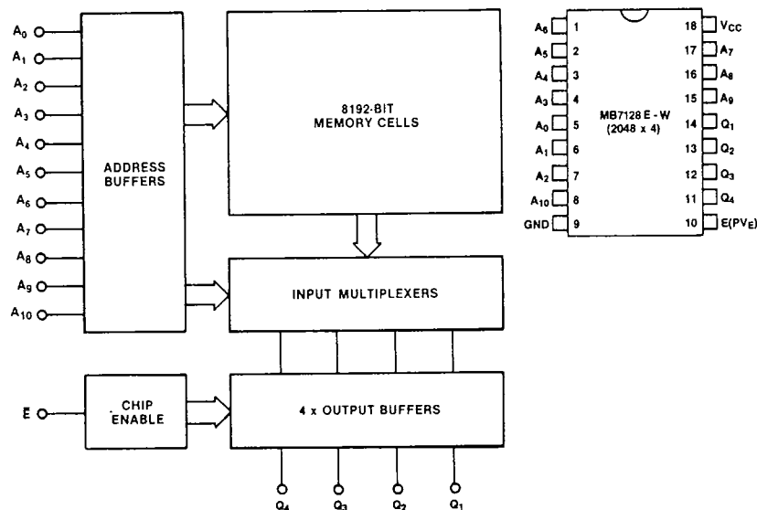
MB7128E-W Block Diagram and Pin Assignment
