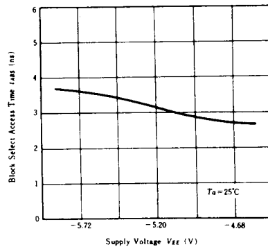
BLOCK SELECT ACCESS TIME vs. SUPPLY VOLTAGE
