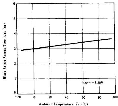
BLOCK SELECT ACCESS TIME vs. AMBIENT TEMPERATURE
