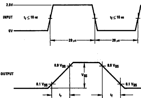
FIGURE 3. Rise Time Control for RS-423
