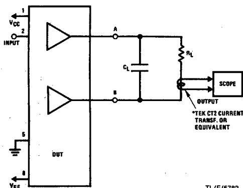
FIGURE 1. Differential Connection
