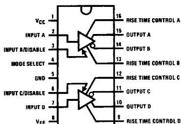
With Mode Select LOW (RS-422 Connection)
