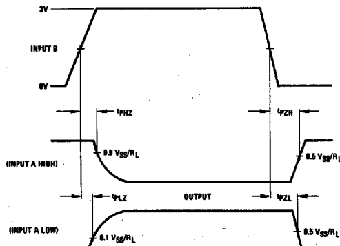
FIGURE 4. TRI-STATE Delays
