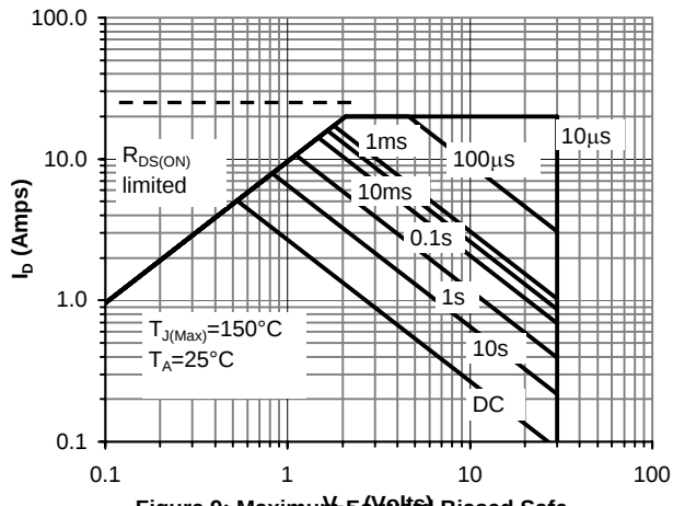
Figure 9: Maximum Allowable Biased Safe Operating Area (Note F)
