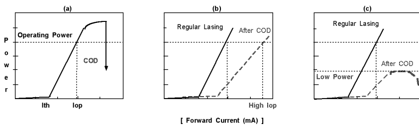
Fig. 1 COD (Catastrophic Optical Damage)
