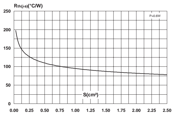
Fig. 11: Thermal resistance junction to ambient versus copper surface under tab (epoxy printed board FR4, Cu = 35µm, typical values).
