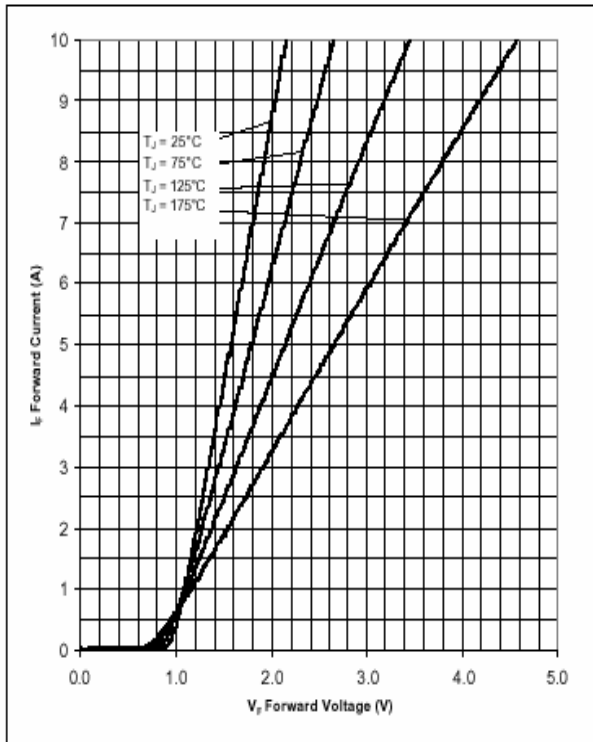
Figure 1. Forward Characteristics
