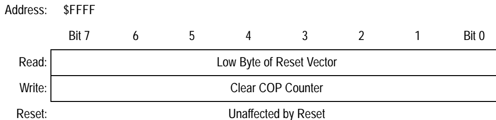
Figure 2. COP Control Register (COPCTL)
