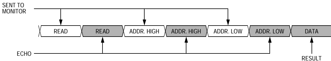
Figure 4. Read Transaction
