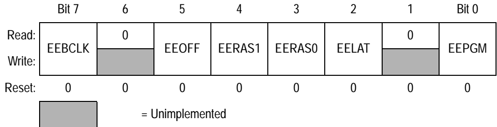
Figure 1. EEPROM-2 Control Register (EECR2)
