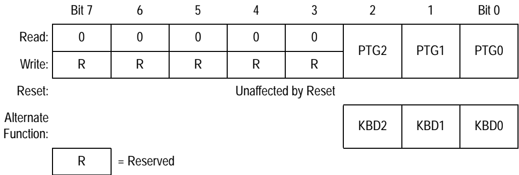
Figure 20. Port G Data Register (PTG)
