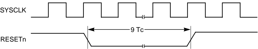
Figure 11.11 Reset Timing
