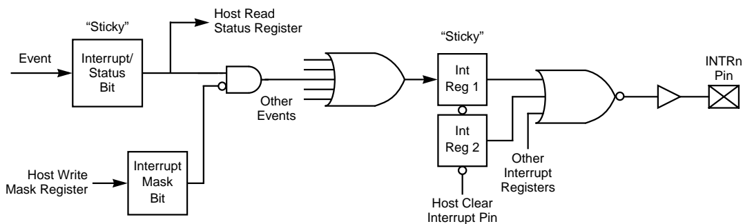
Figure 5.7 Interrupt Structure
