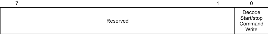
Figure 4.85 Register 246 (0x0F6)
