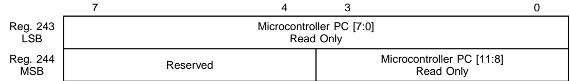
Figure 4.83 Register 243 and 244 (0x0F3 and 0x0F4) Microcontroller PC [11:0]
