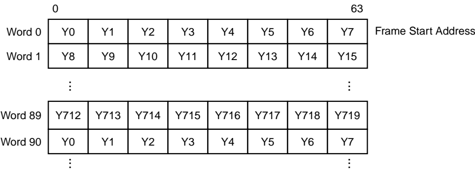
Figure 7.5 Luma Frame Store Organization
