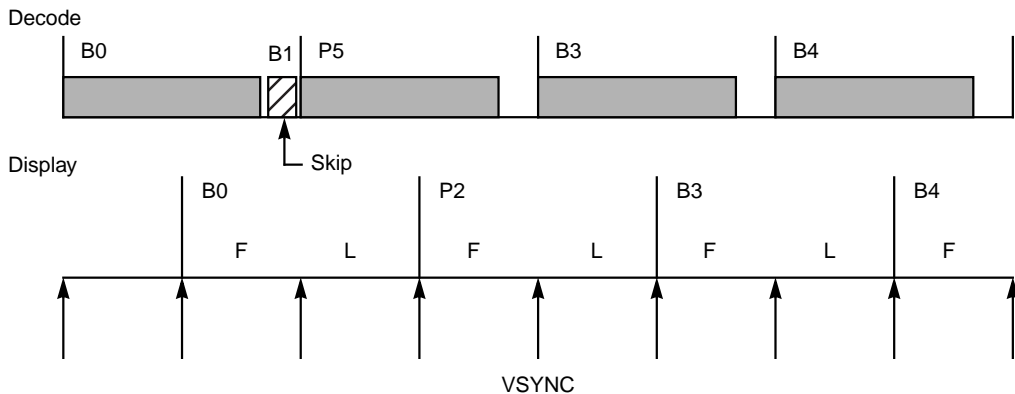
Figure 8.5 Single Skip with and without Display Freeze
