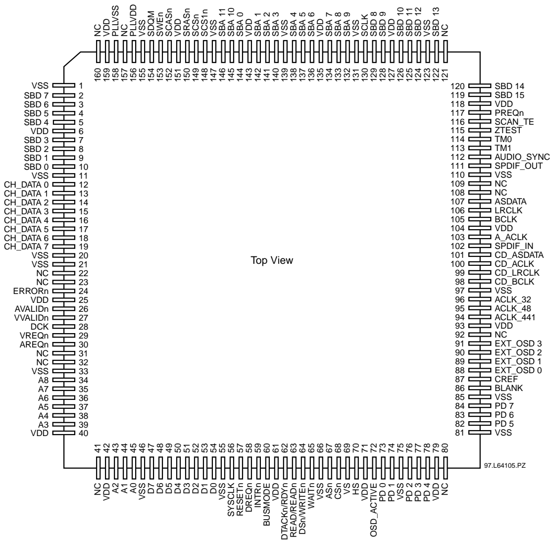
Figure 11.16 160-Pin Package Pinout
