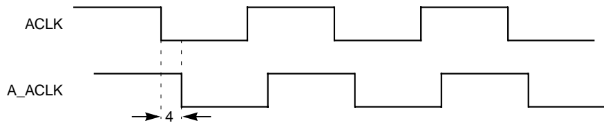
Figure 11.14 A_ACLK Timing
