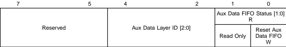
Figure 4.17 Register 64 (0x040)
