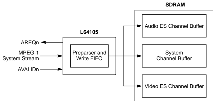
Figure 6.8 Preparing an MPEG-1 System Stream
