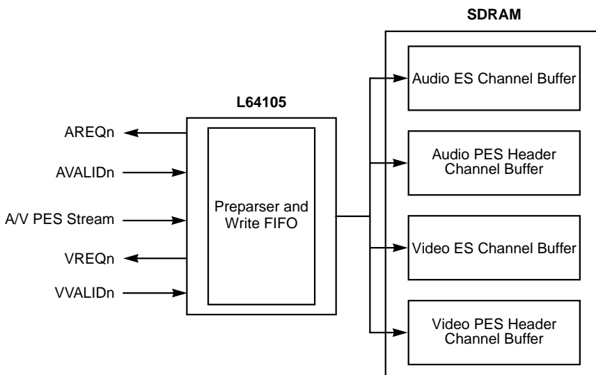
Figure 6.14 Parsing an Audio/Video PES Transport Stream
