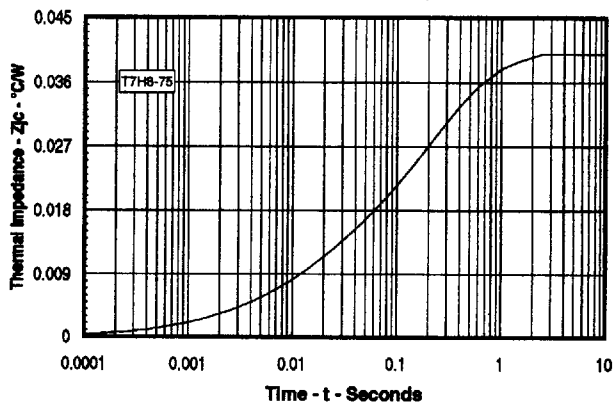
Maximum Transient Thermal Impedance
