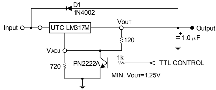
Figure 1. 1.5V Electronic Shutdown Regulator D1 protects the device during an input short circuit
