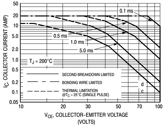
Figure 6. 2N6052, 2N6059
