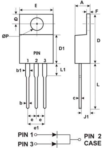
TO-220AB
