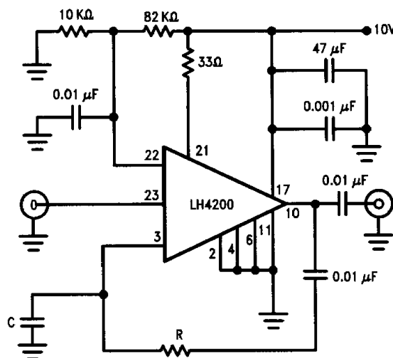
FIGURE 5. Feedback Amplifier
