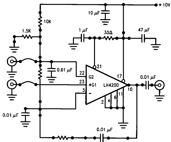
FIGURE 2. Applications Board
