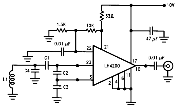
FIGURE 3. VHF-UHF Oscillator
