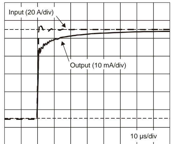
Figure 16: Typical di/dt follow-up (low speed 1 turn PCB design)
