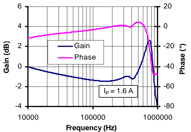
Figure 13: Typical frequency response (low speed 1 turn PCB design) ( I_p = 1.6 A )
