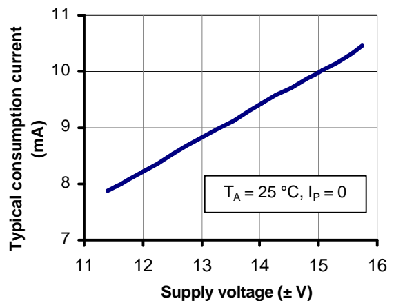
Figure 7: Consumption current
