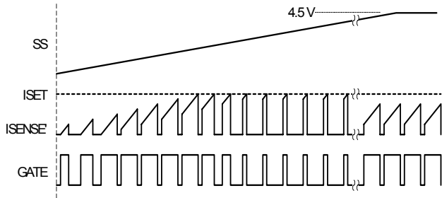
FIGURE 6. PULSE-BY-PULSE OC BEHAVIOR DURING SS
