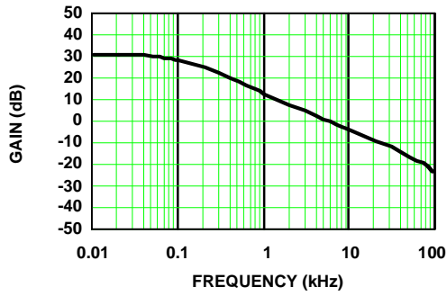
FIGURE 12A. GAIN
