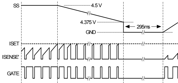
FIGURE 7. OC SHUTDOWN BEHAVIOR
