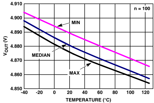
FIGURE 58. V OUT HIGH vs TEMPERATURE R L = 1k. V S = ±2.5V
