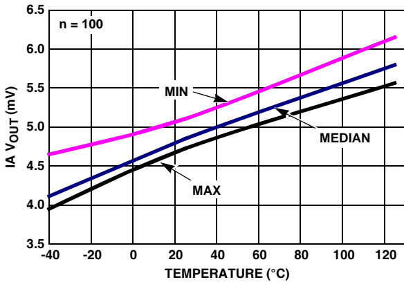
FIGURE 57. IA V OUT LOW vs TEMPERATURE R L = 100k. V S = ±2.5V
