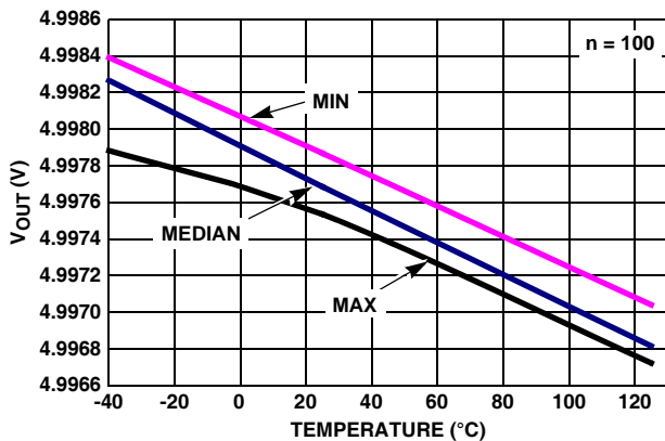
FIGURE 59. V OUT HIGH vs TEMPERATURE R L = 100k. V S = ±2.5V
