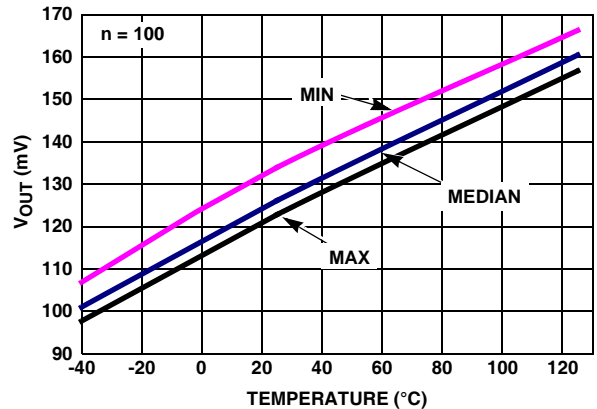
FIGURE 60. V OUT LOW vs TEMPERATURE R L = 1k. V S = ±2.5V
