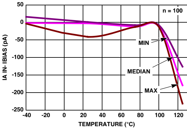
FIGURE 37. I BIAS (IA IN-) vs TEMPERATURE V_S = \pm 1.2V
