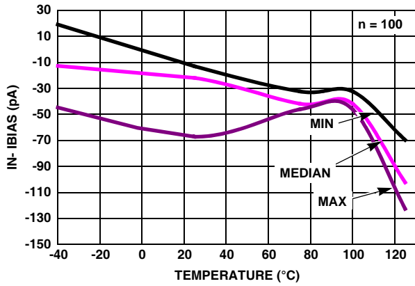
FIGURE 39. I BIAS(IN-) vs TEMPERATURE V_S = \pm 2.5V
