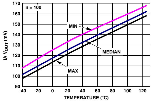
FIGURE 56. IA V OUT LOW vs TEMPERATURE R L = 1k. V S = ±2.5V
