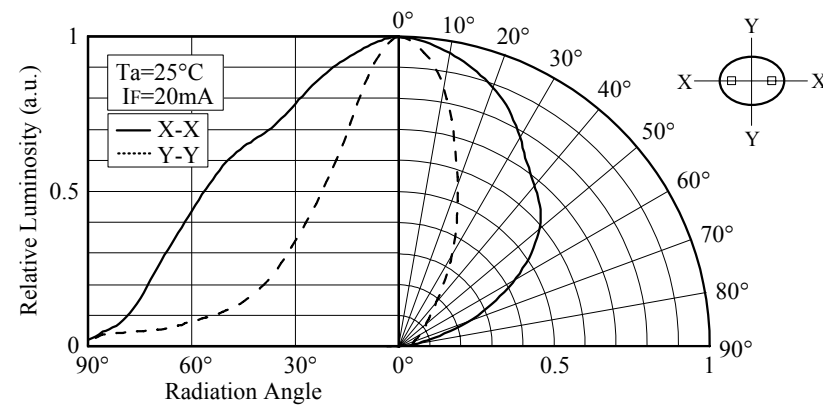
■ Directivity (NSPB546BS)
