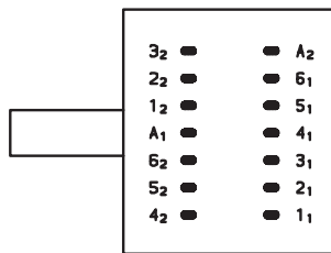
2 POLES 2 - 6 POSITIONS
