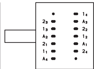
4 CIRCUITS 2 POSITIONS
