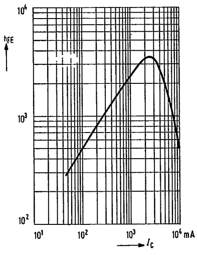
DC current gain h_{FE} = f(I_C) V_{CE} = 3\text{ V}; T_{case} = 25^\circ\text{C} BD 644, BD 646, BD 648, BD 650
