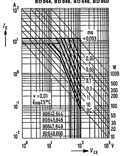
Permissible operating range I_C = f(V_{CE}); T_{case} = 25^\circ\text{C}, v = 0.01 BD 644, BD 646, BD 648, BD 650
