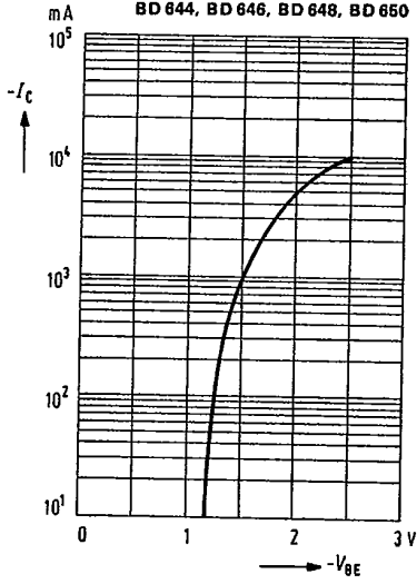
Collector current I_C = f(V_{BE}) -V_{CE} = 3V; T_{case} = 25^\circ C BD 644, BD 646, BD 648, BD 650
