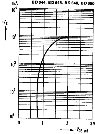
Collector-emitter saturation voltage V_{CEsat} = f(I_C); h_{FE} = 250; T_{case} = 25^\circ C BD 644, BD 646, BD 648, BD 650
