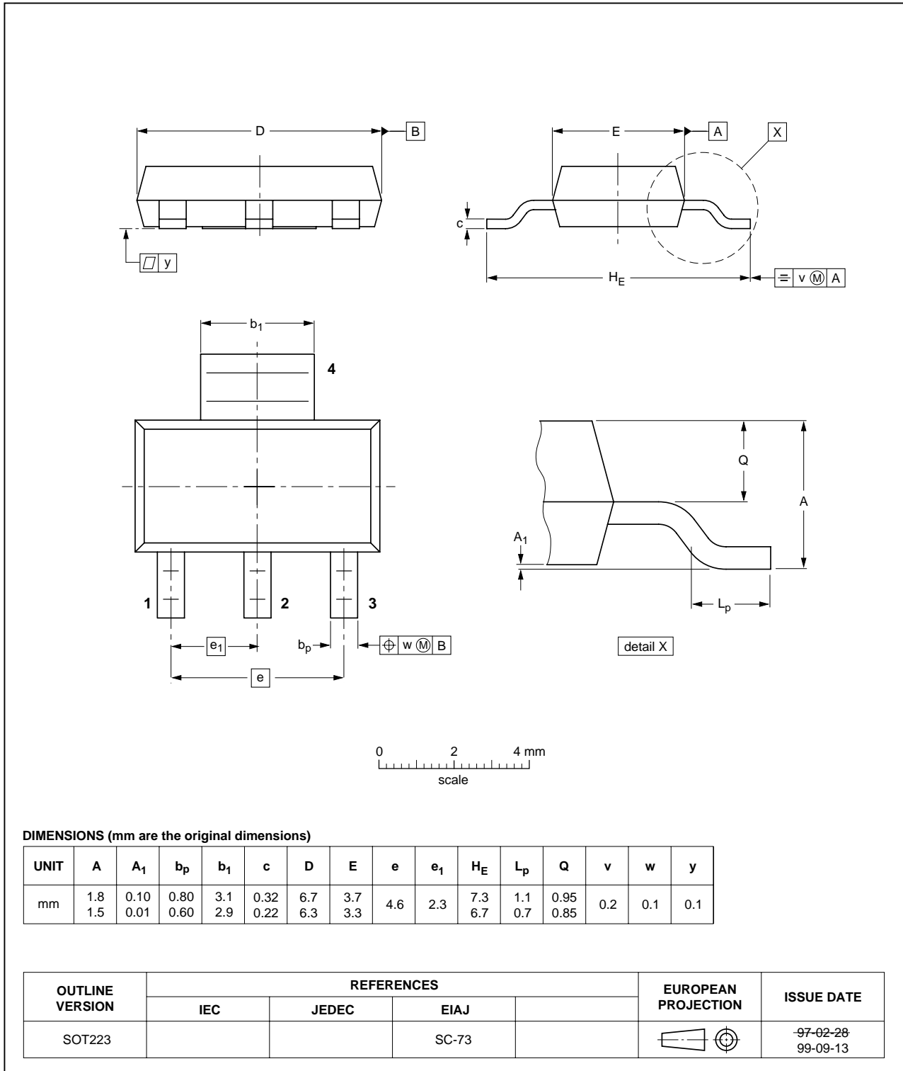
Fig 15. Package outline.
