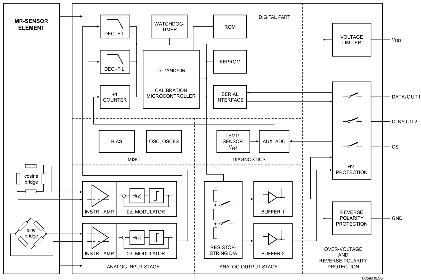
Fig 1. Functional diagram
