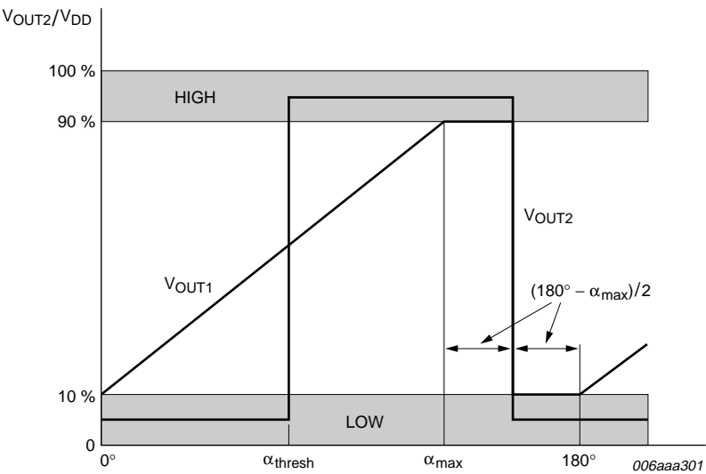
Fig 6. Comparator analog output (mode 3)
