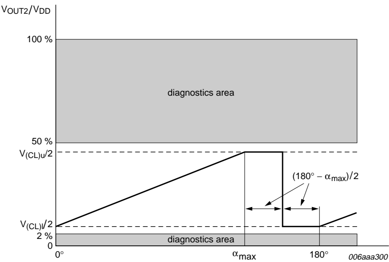
Fig 5. Half range output mode (mode 2)
