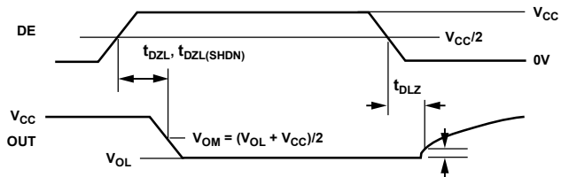
Figure 11. Driver Enable and Disable Times ( t_{DZL} , t_{DLZ} , t_{DZL(SHDN)} )
