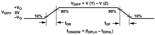
Figure 9. Driver Propagation Delays
