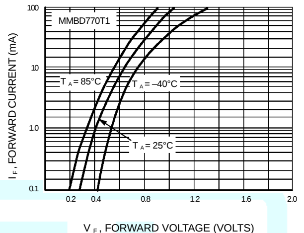
Figure 4. Forward Voltage
