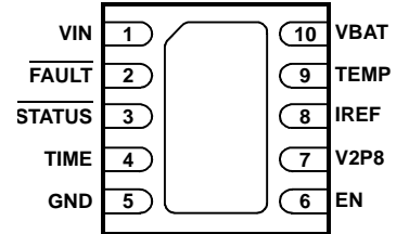
ISL9205D (10 LD DFN) TOP VIEW
