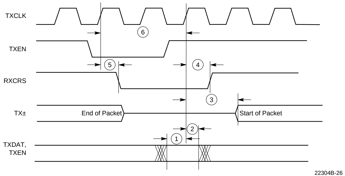
Figure 2. 10 Mbps Transmit Timing (GPSI)
