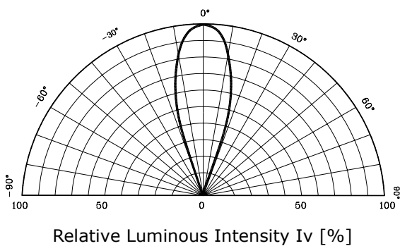
Fig. 5-1 Radiation Diagram(X)
