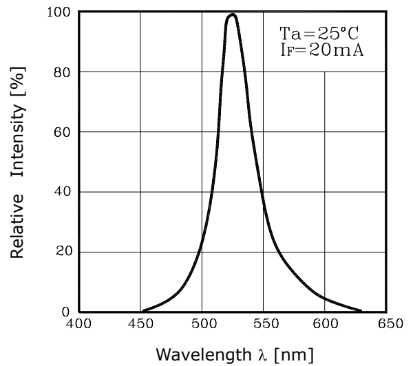
Fig.4 Spectrum Distribution
