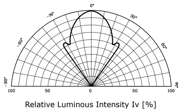
Fig. 5-2 Radiation Diagram(Y)
