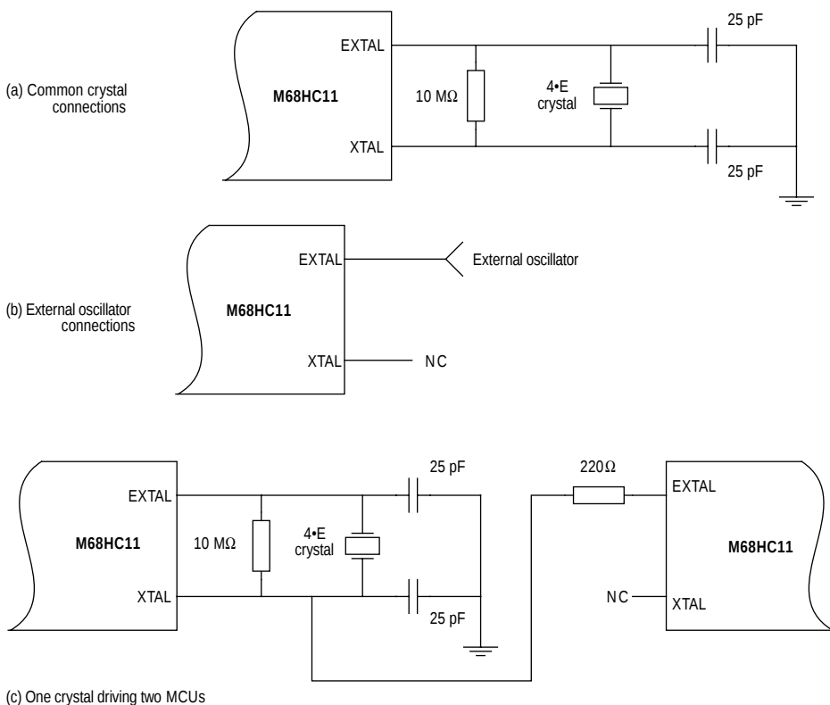
Figure 2-3 Oscillator connections
